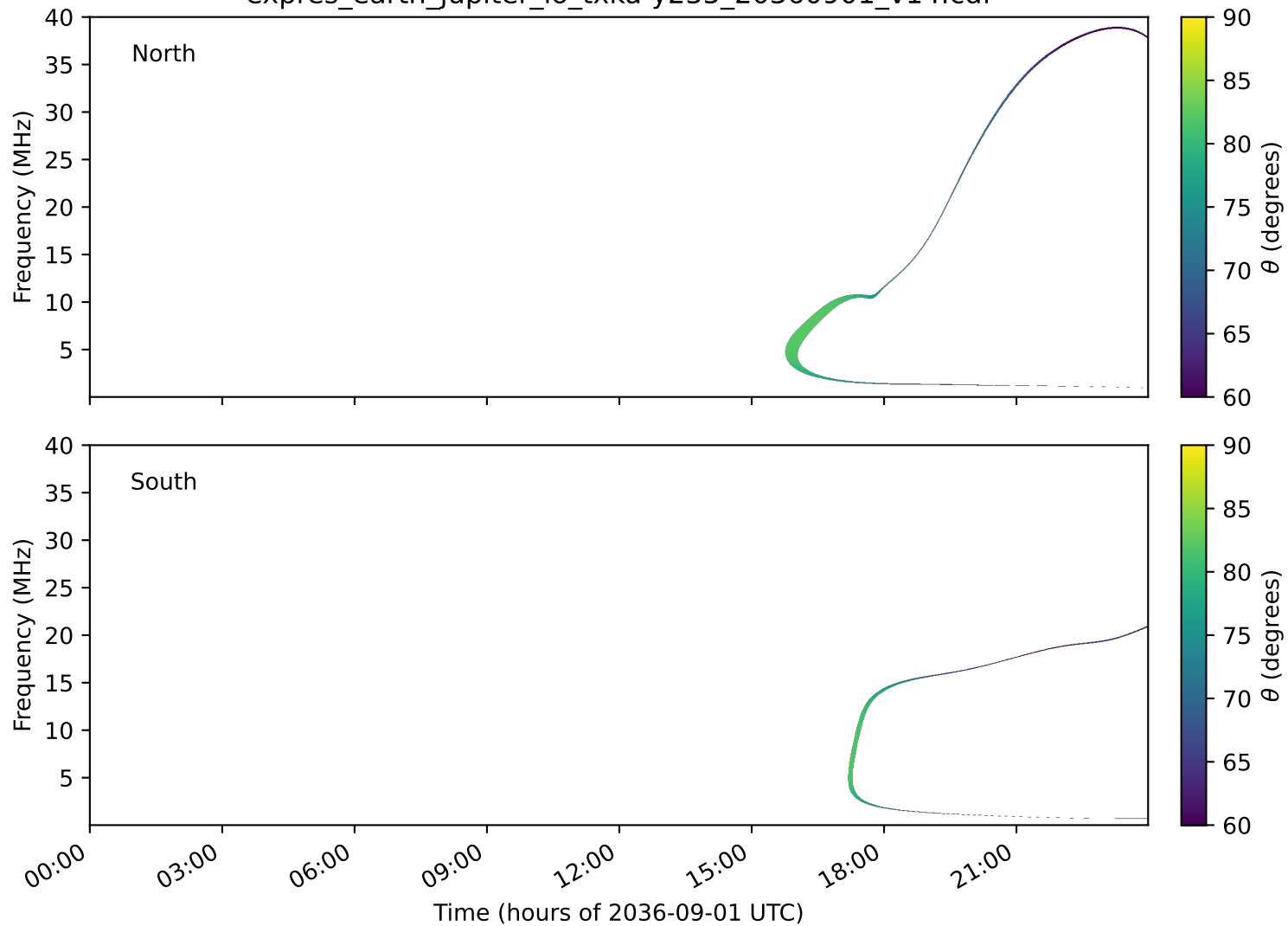
expres_earth_jupiter_io_txka-y235_20360901_v14.cdf
