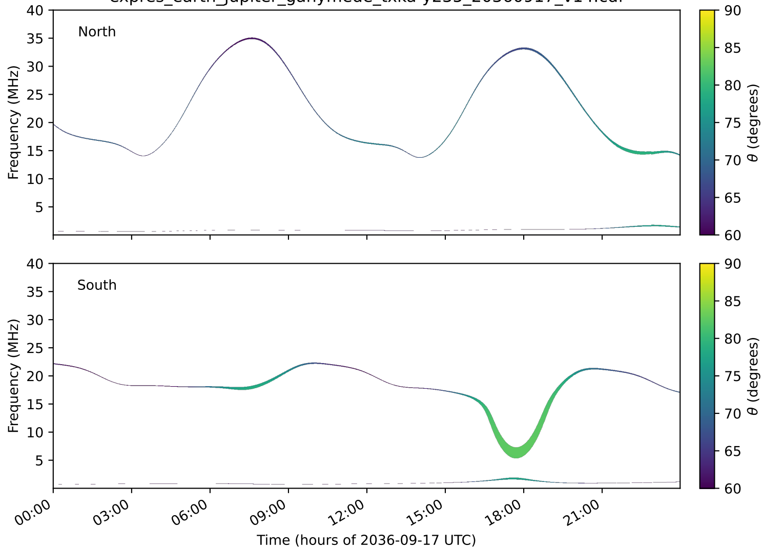
expres_earth_jupiter_ganymede_txka-y235_20360917_v14.cdf
