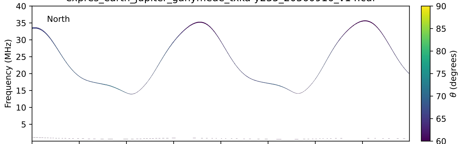
expres_earth_jupiter_ganymede_txka-y235_20360916_v14.cdf
