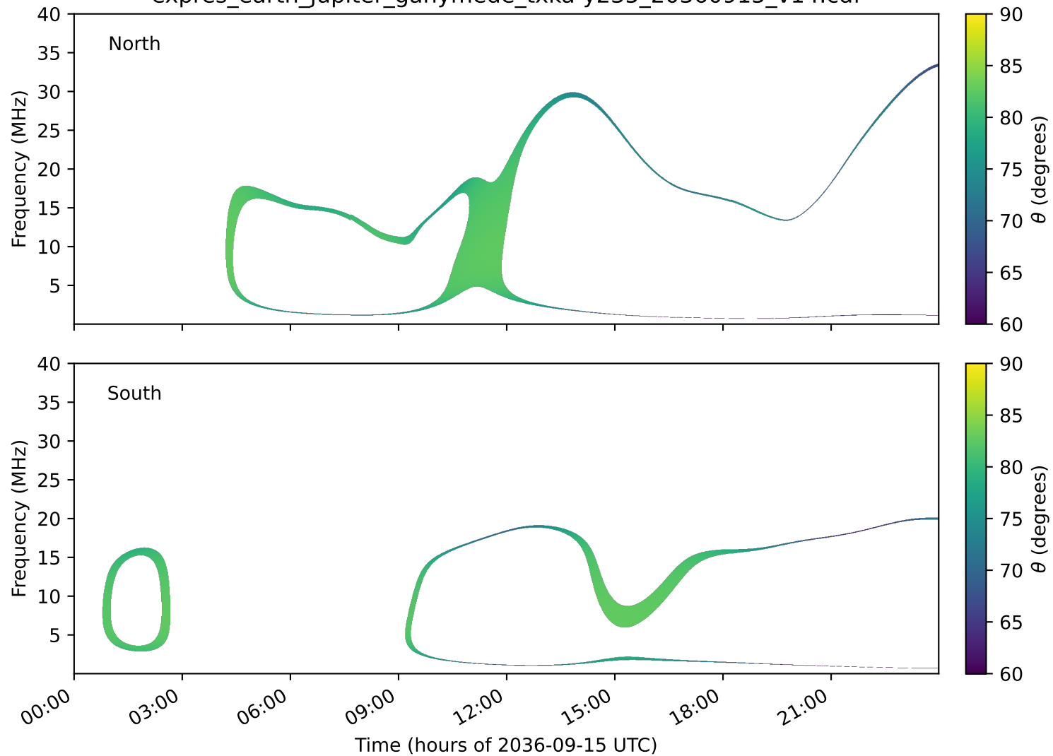
expres_earth_jupiter_ganymede_txka-y235_20360915_v14.cdf
