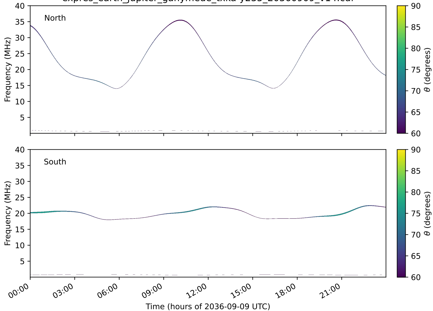
expres_earth_jupiter_ganymede_txka-y235_20360909_v14.cdf
