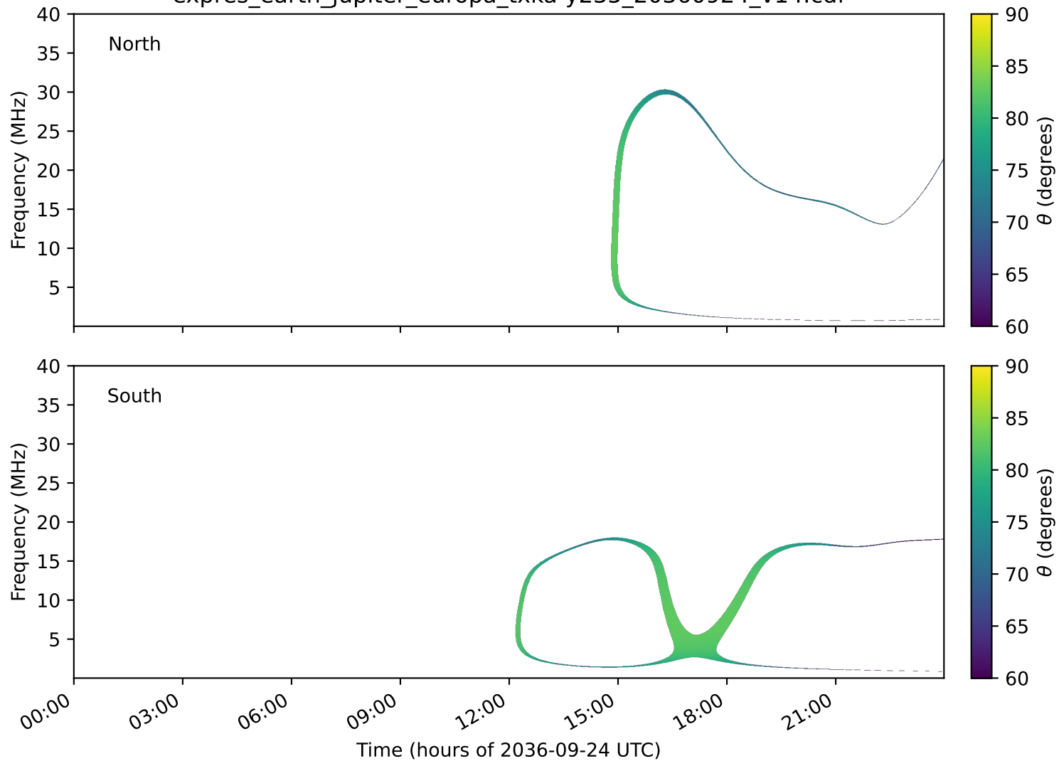
expres_earth_jupiter_europa_txka-y235_20360924_v14.cdf
