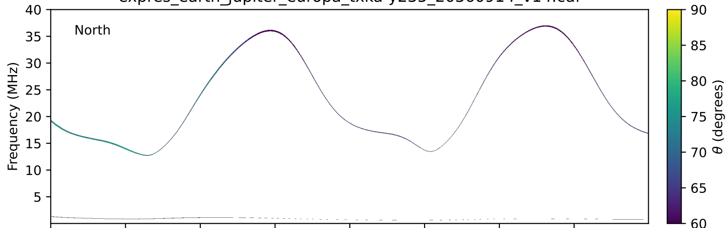
expres_earth_jupiter_europa_txka-y235_20360914_v14.cdf
