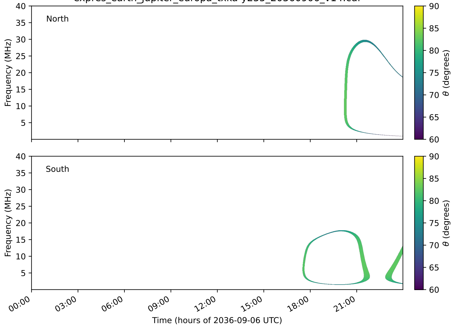
expres_earth_jupiter_europa_txka-y235_20360906_v14.cdf
