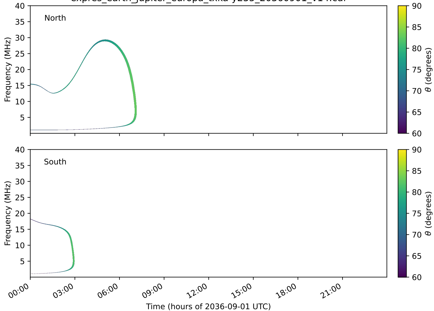
expres_earth_jupiter_europa_txka-y235_20360901_v14.cdf
