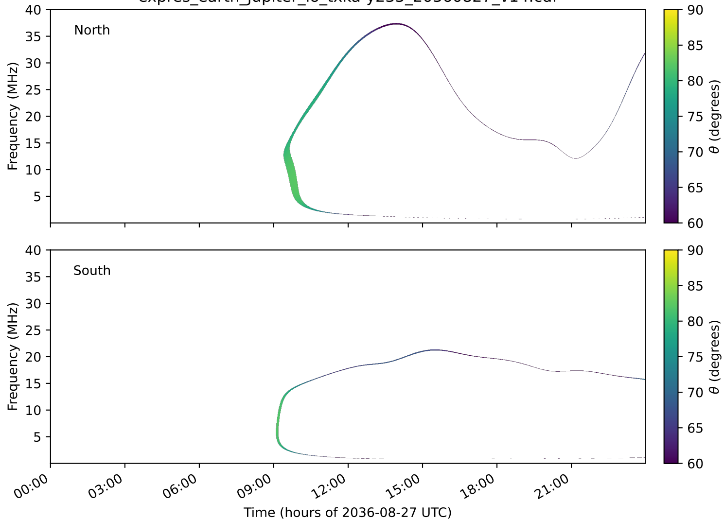
expres_earth_jupiter_io_txka-y235_20360827_v14.cdf
