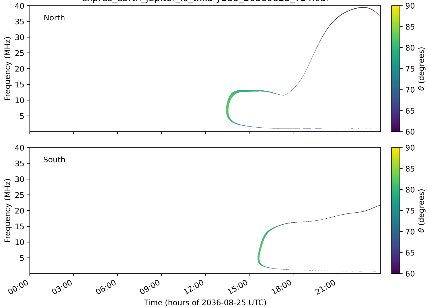
expres_earth_jupiter_io_txka-y235_20360825_v14.cdf
