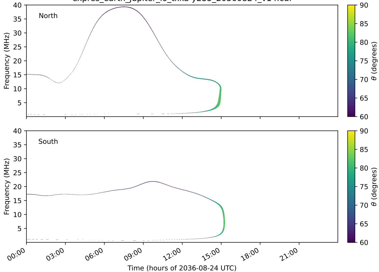
expres_earth_jupiter_io_txka-y235_20360824_v14.cdf
