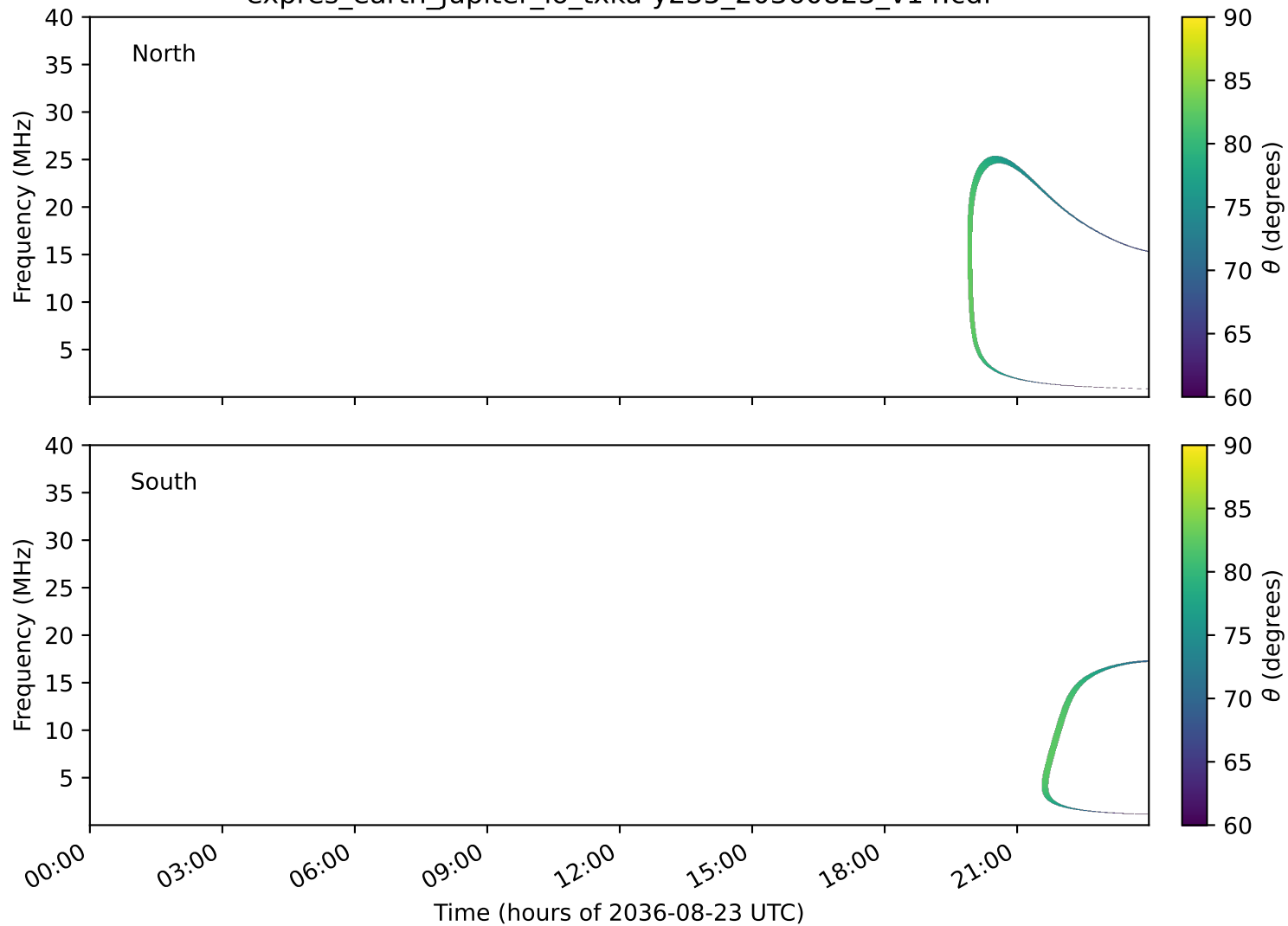
expres_earth_jupiter_io_txka-y235_20360823_v14.cdf
