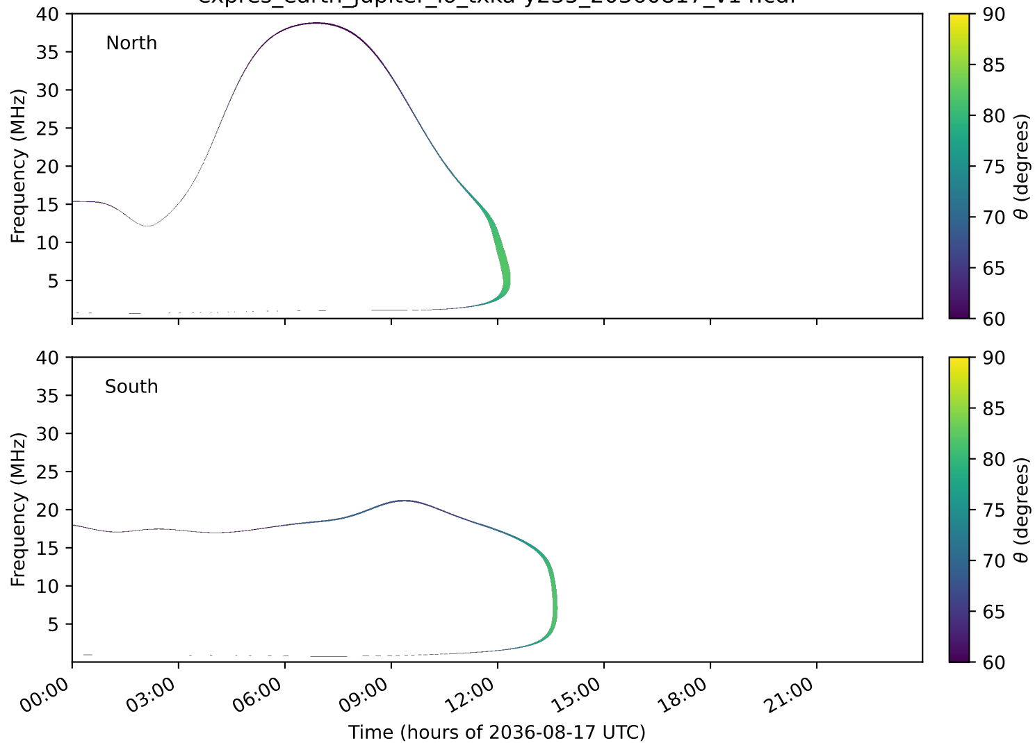
expres_earth_jupiter_io_txka-y235_20360817_v14.cdf
