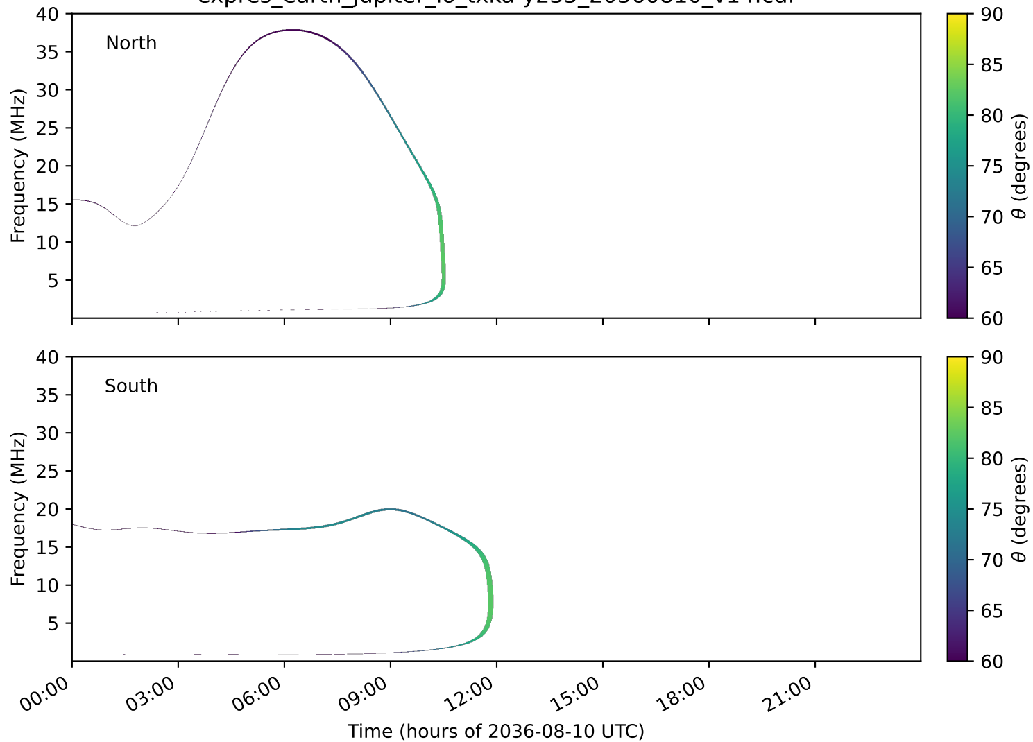
expres_earth_jupiter_io_txka-y235_20360810_v14.cdf
