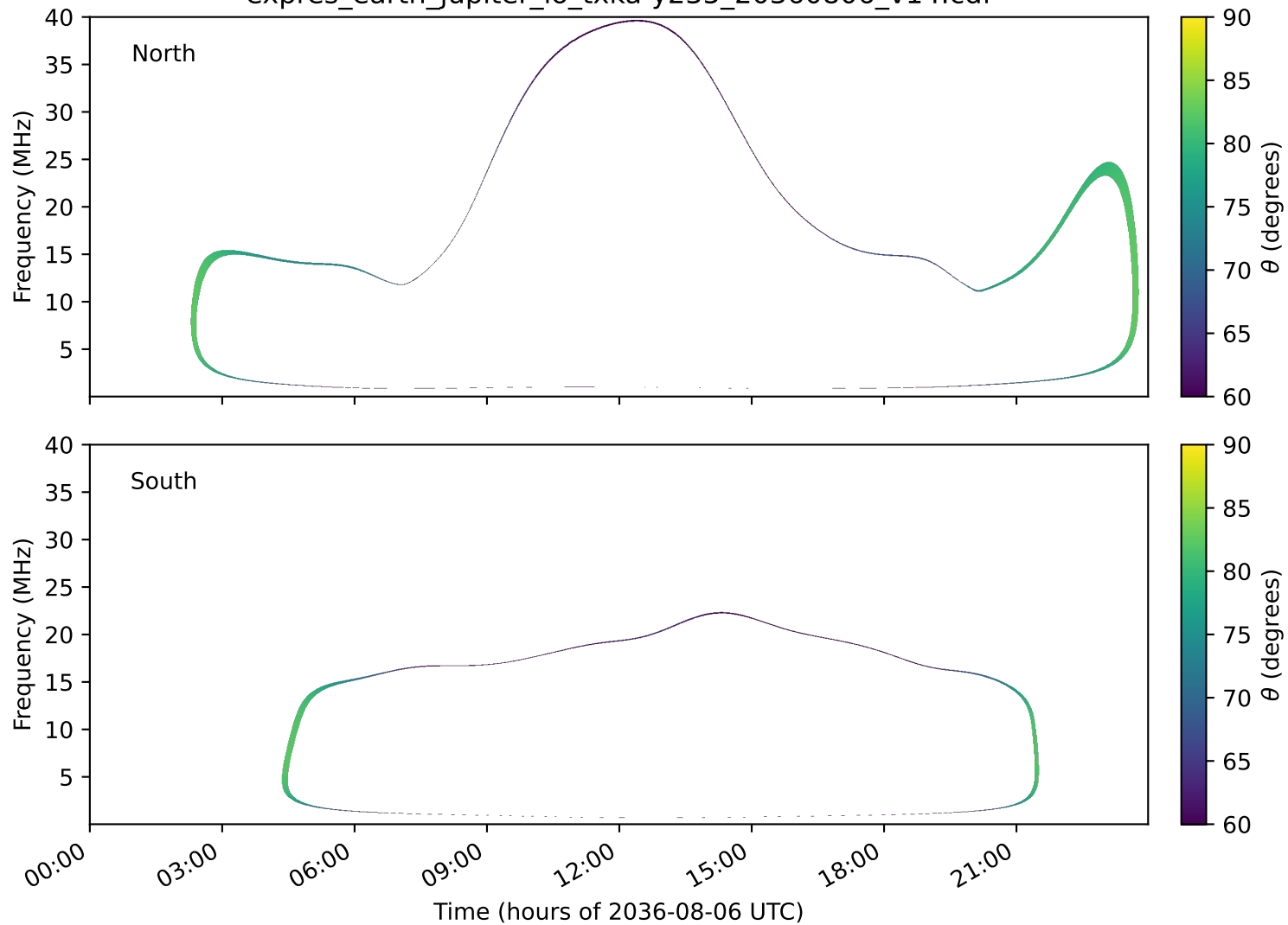
expres_earth_jupiter_io_txka-y235_20360806_v14.cdf
