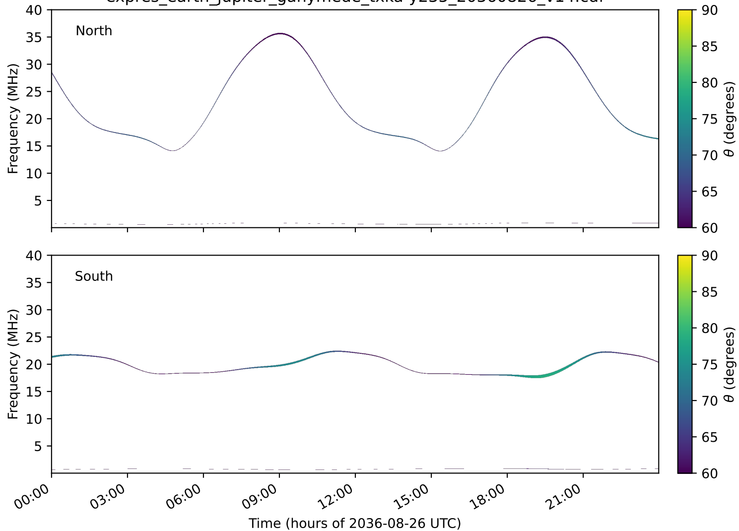
expres_earth_jupiter_ganymede_txka-y235_20360826_v14.cdf
