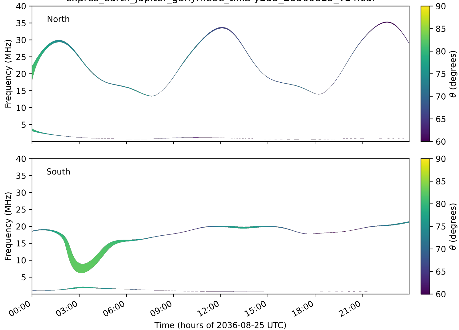
expres_earth_jupiter_ganymede_txka-y235_20360825_v14.cdf
