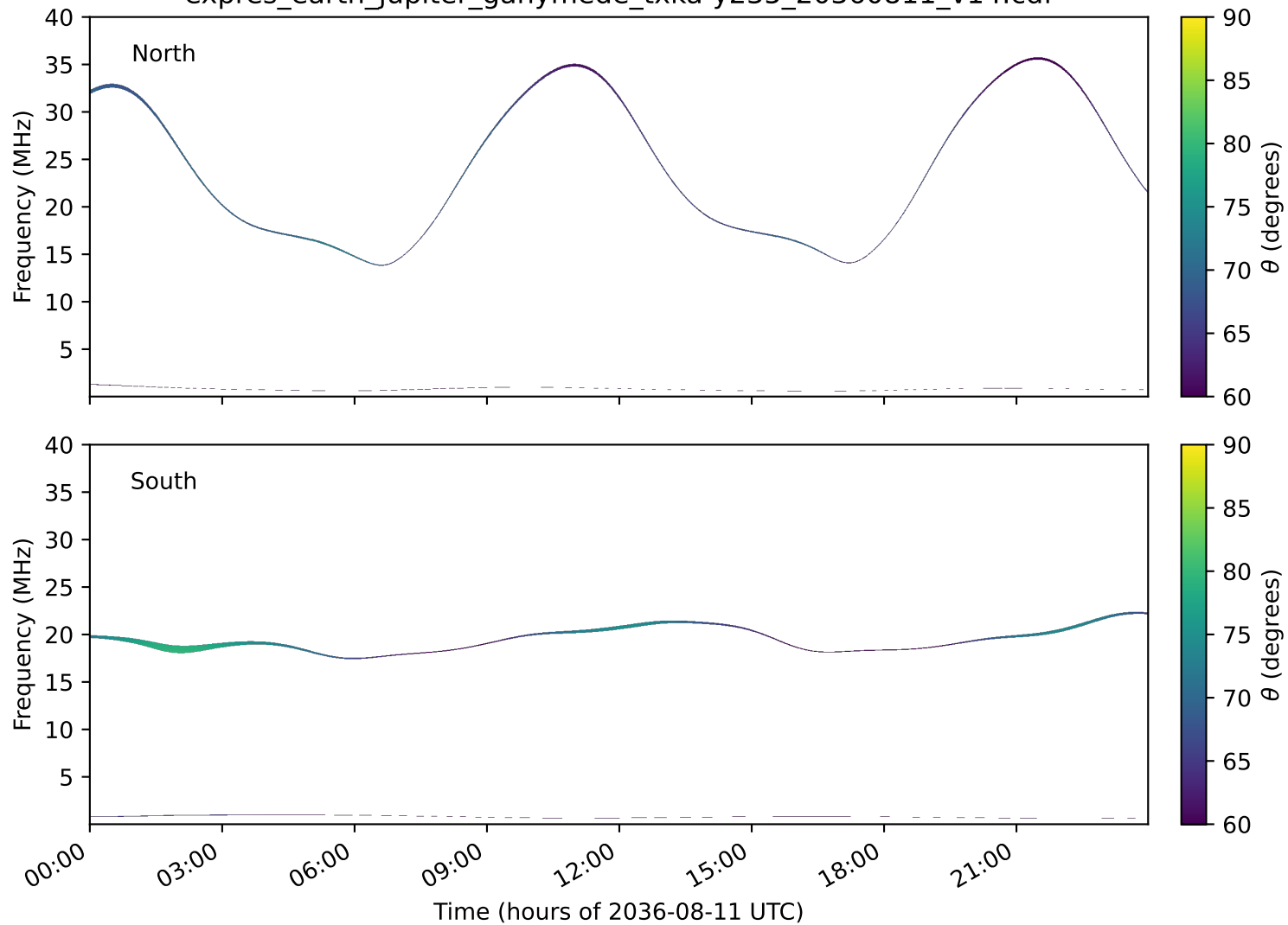
expres_earth_jupiter_ganymede_txka-y235_20360811_v14.cdf
