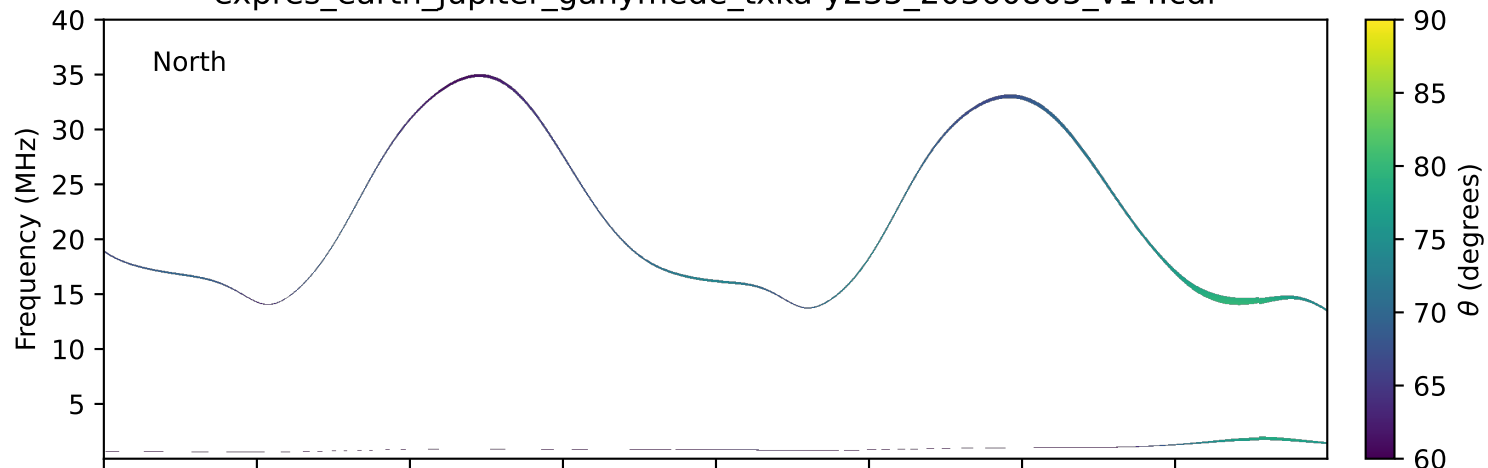
expres_earth_jupiter_ganymede_txka-y235_20360805_v14.cdf
