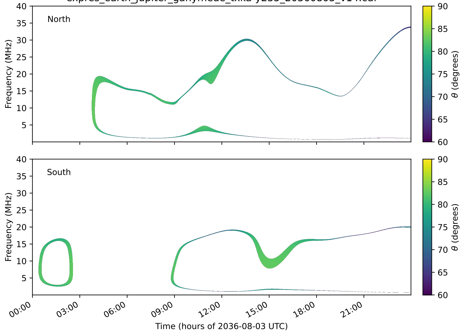
expres_earth_jupiter_ganymede_txka-y235_20360803_v14.cdf
