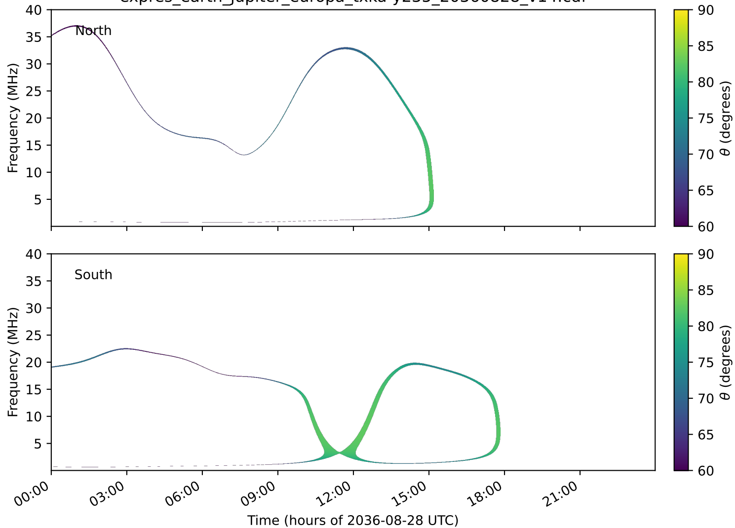
expres_earth_jupiter_europa_txka-y235_20360828_v14.cdf
