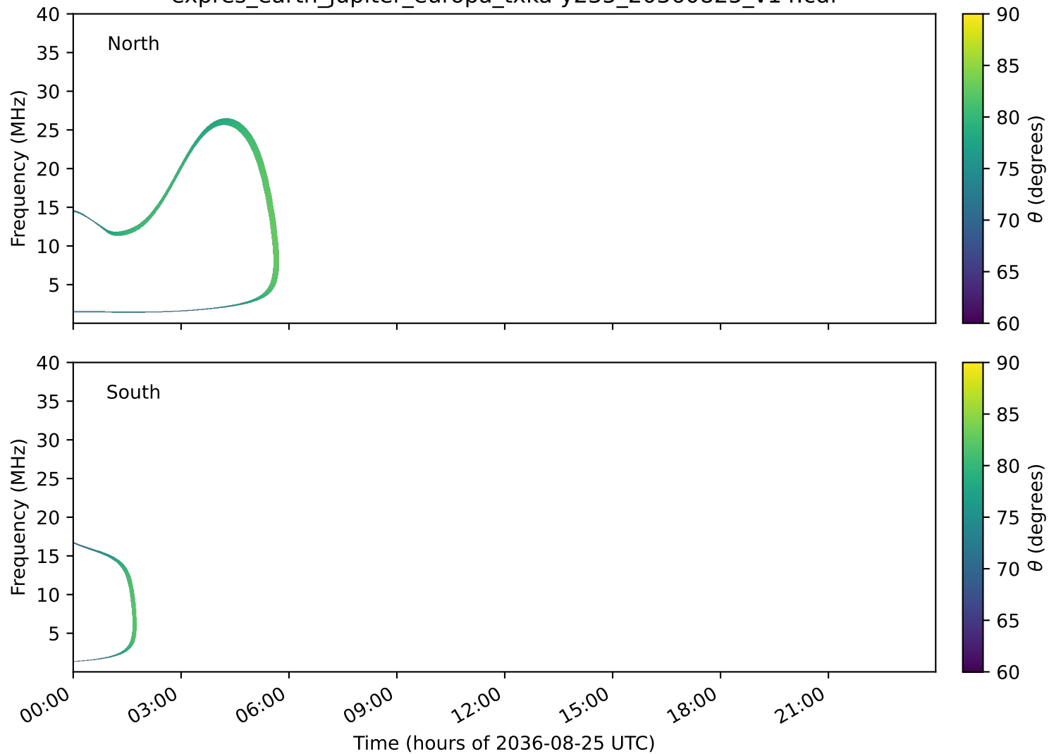
expres_earth_jupiter_europa_txka-y235_20360825_v14.cdf
