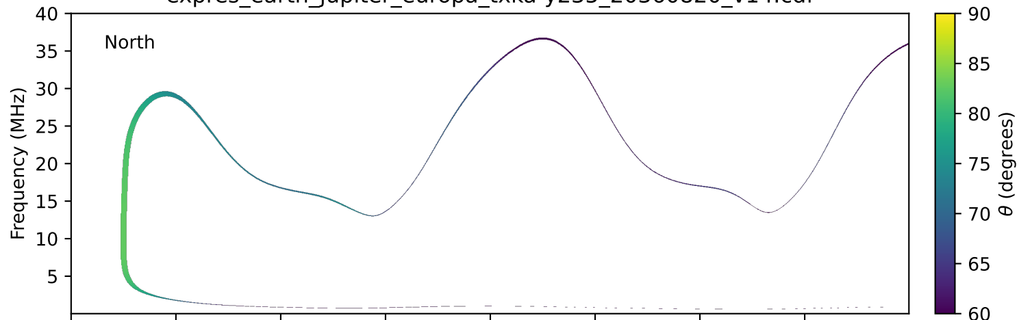
expres_earth_jupiter_europa_txka-y235_20360820_v14.cdf
