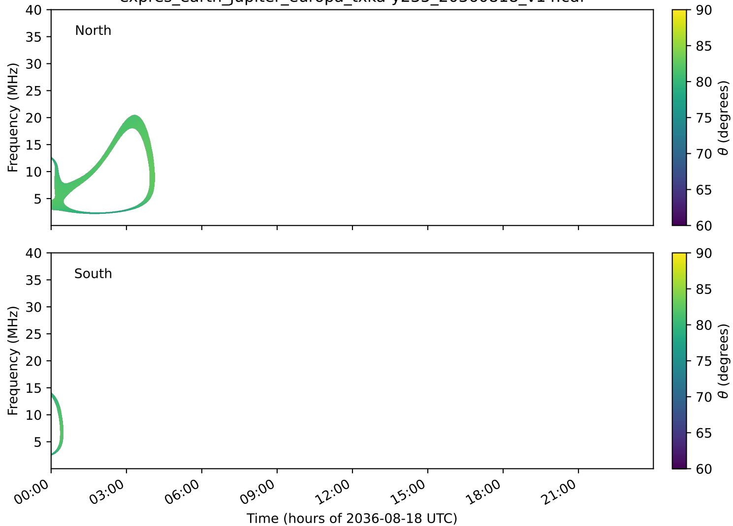
expres_earth_jupiter_europa_txka-y235_20360818_v14.cdf
