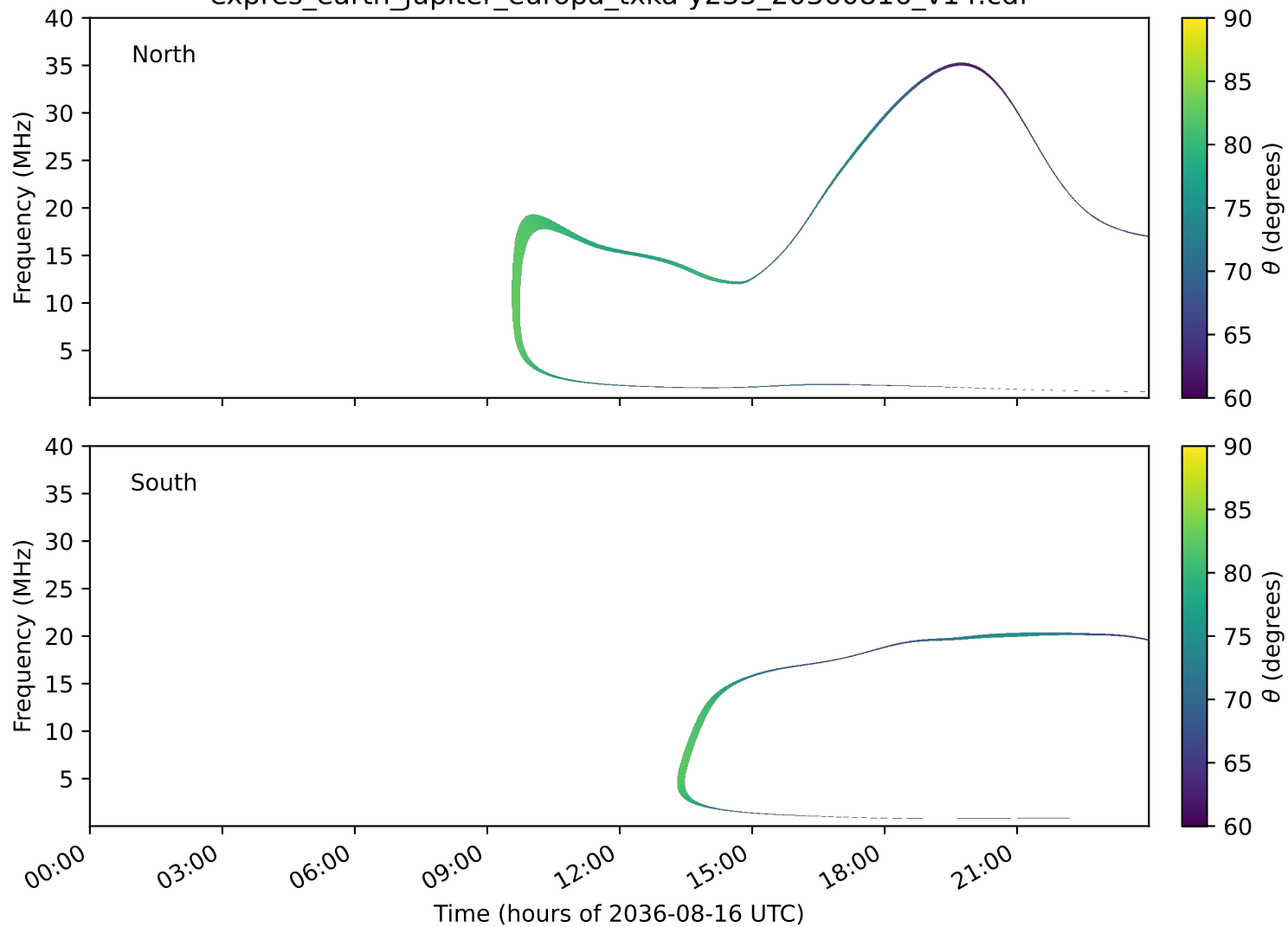
expres_earth_jupiter_europa_txka-y235_20360816_v14.cdf
