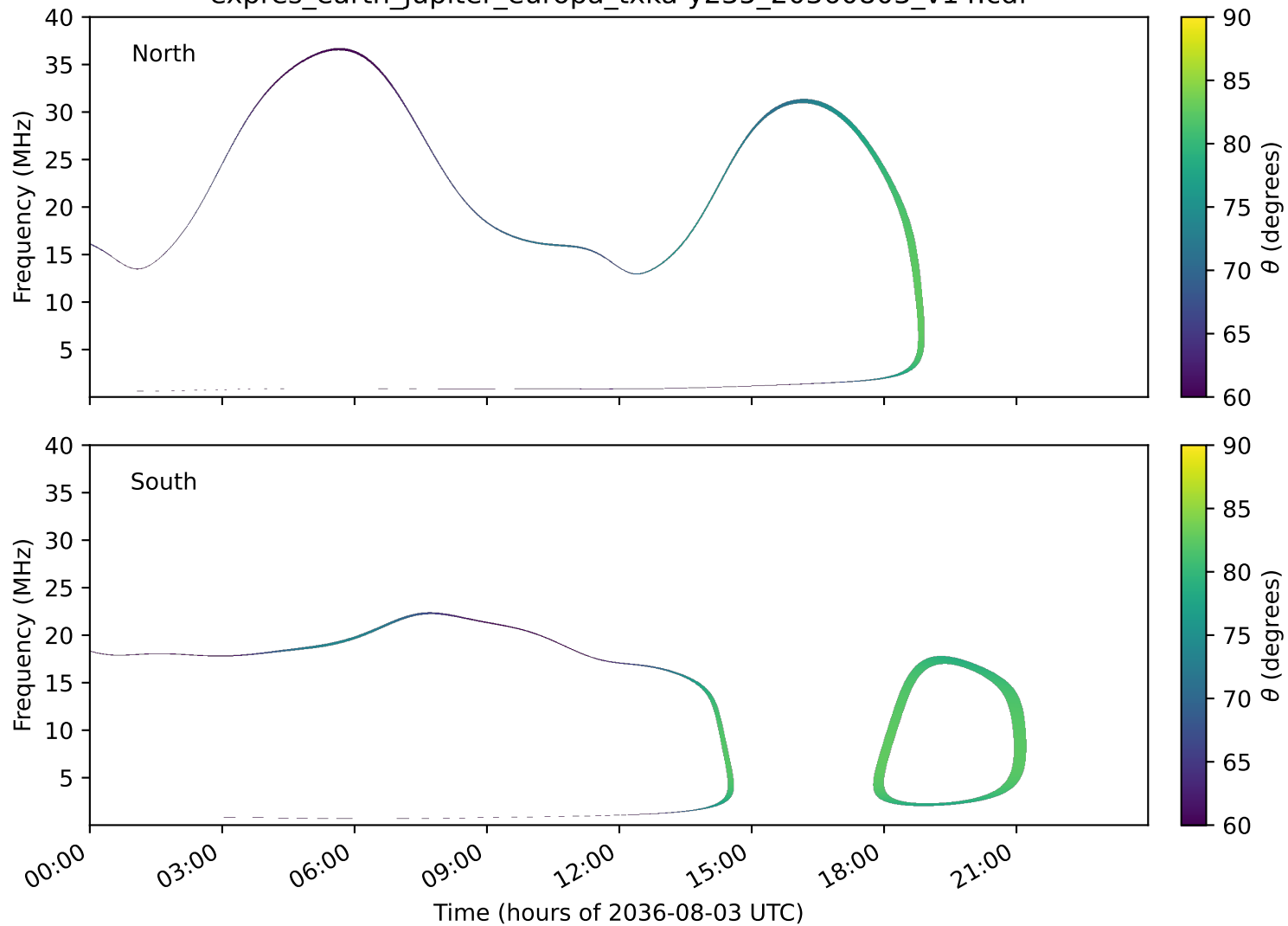
expres_earth_jupiter_europa_txka-y235_20360803_v14.cdf
