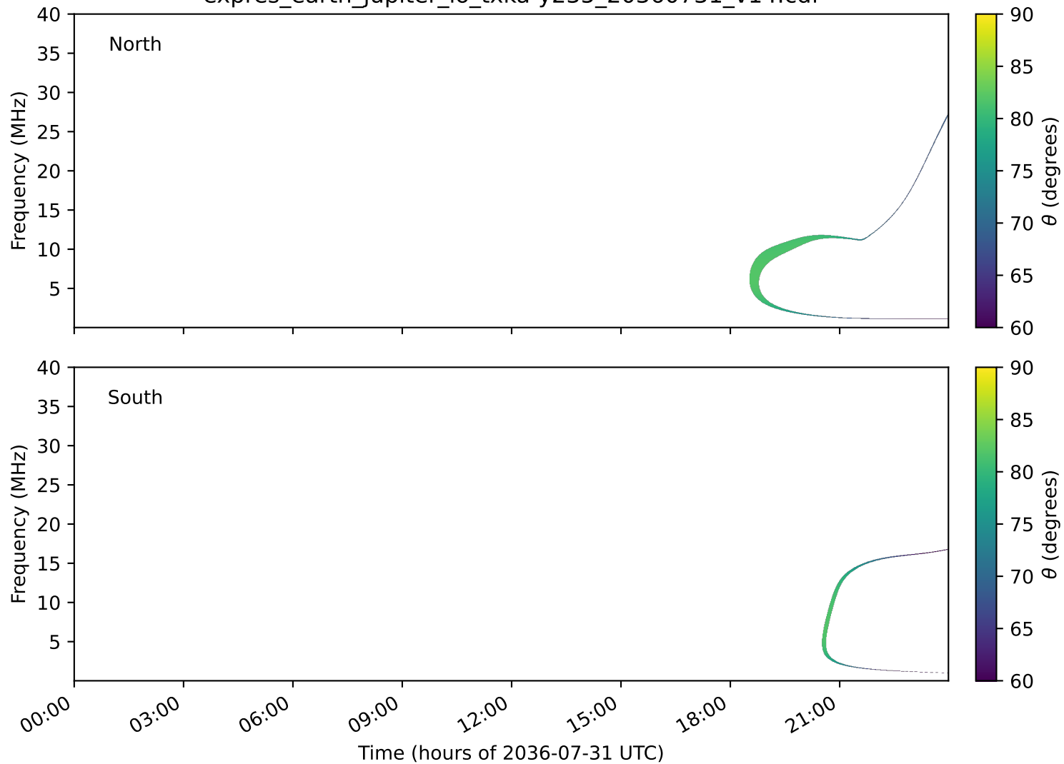
expres_earth_jupiter_io_txka-y235_20360731_v14.cdf
