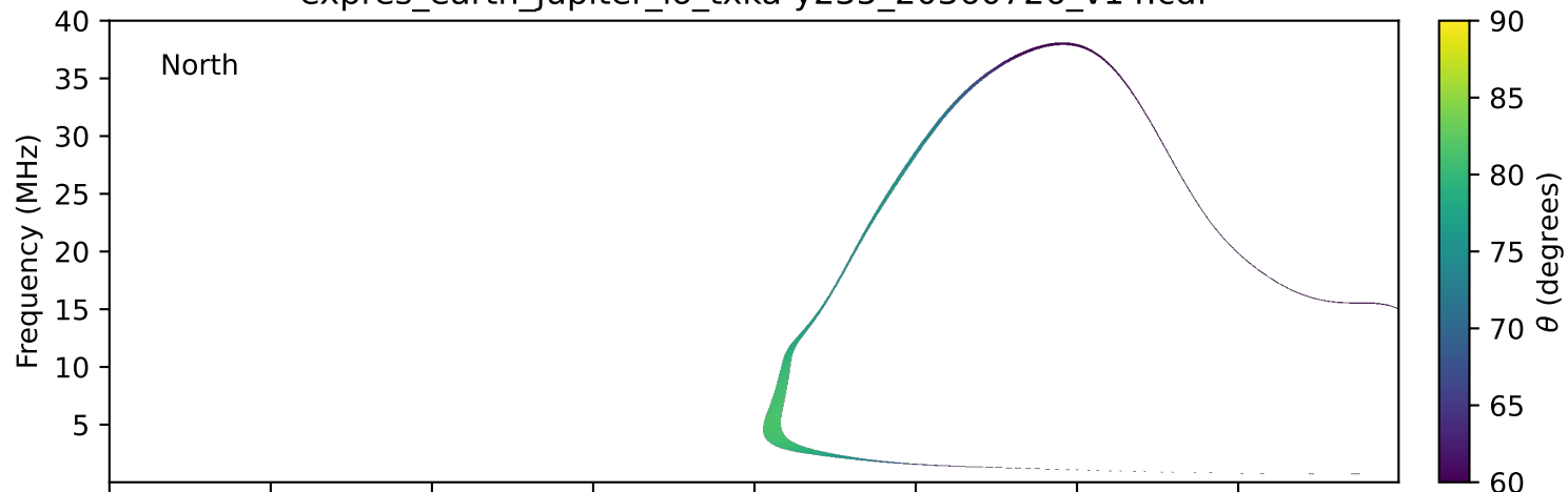
expres_earth_jupiter_io_txka-y235_20360726_v14.cdf
