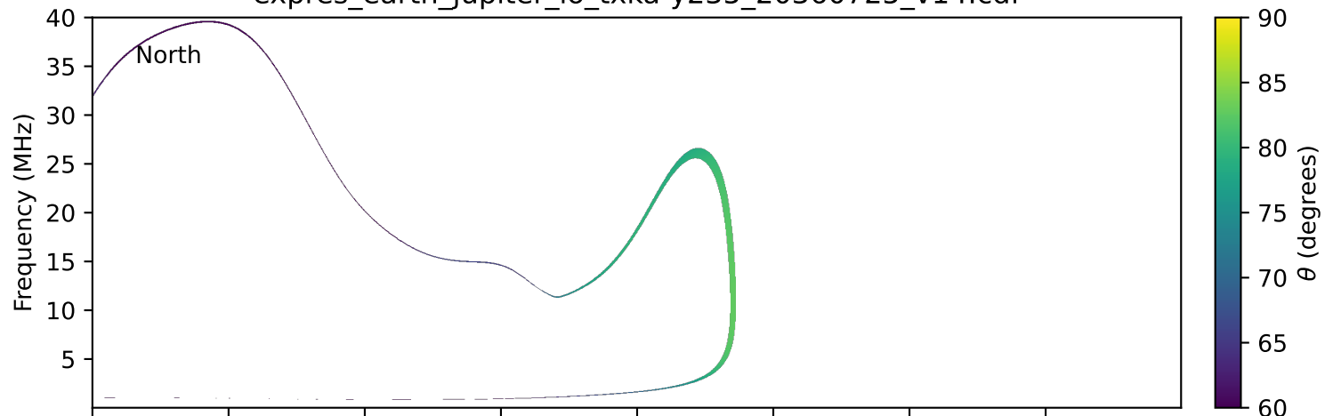
expres_earth_jupiter_io_txka-y235_20360725_v14.cdf
