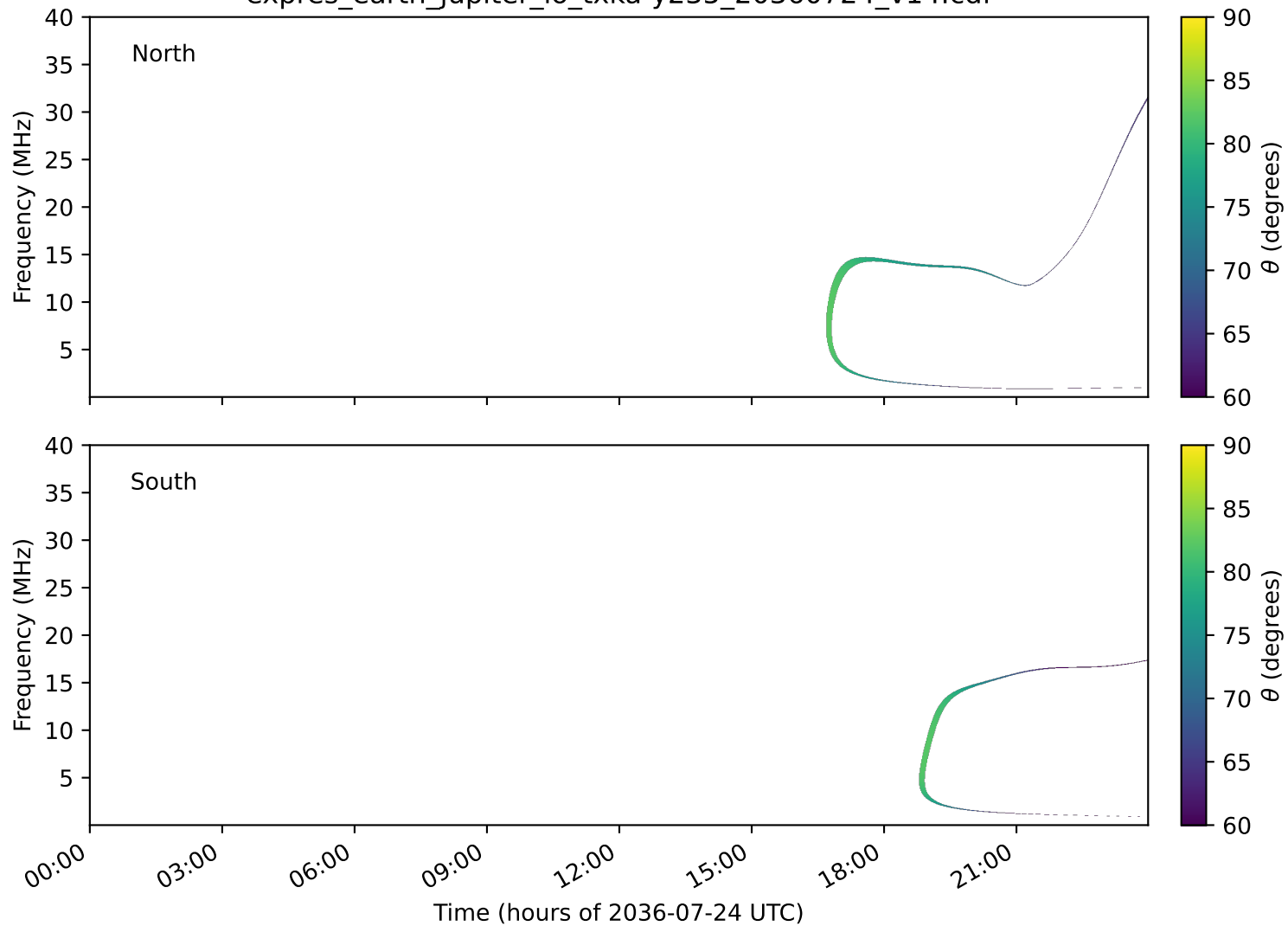
expres_earth_jupiter_io_txka-y235_20360724_v14.cdf
