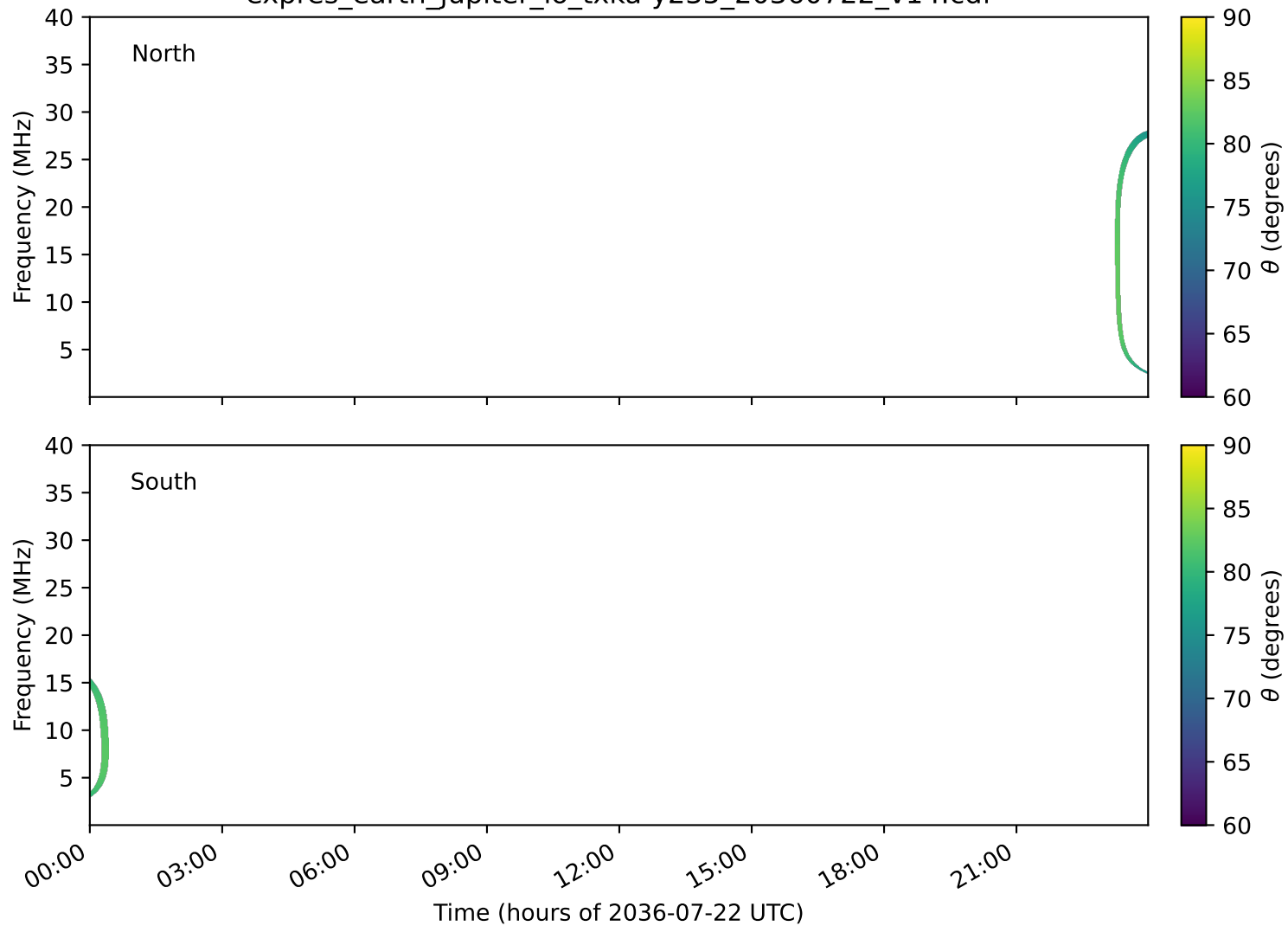
expres_earth_jupiter_io_txka-y235_20360722_v14.cdf
