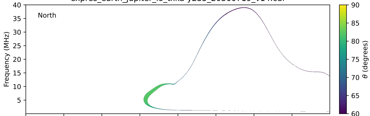
expres_earth_jupiter_io_txka-y235_20360719_v14.cdf
