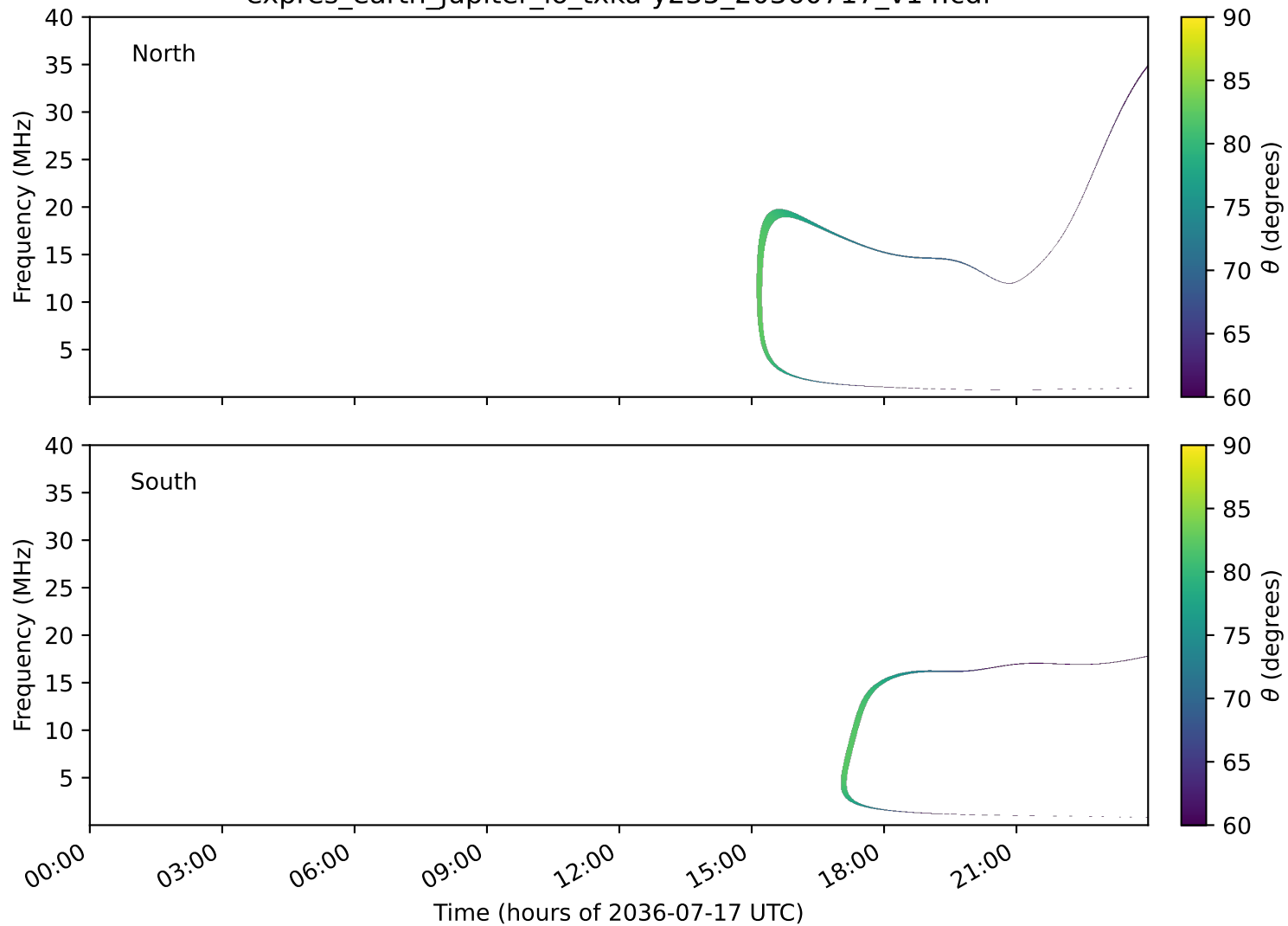
expres_earth_jupiter_io_txka-y235_20360717_v14.cdf
