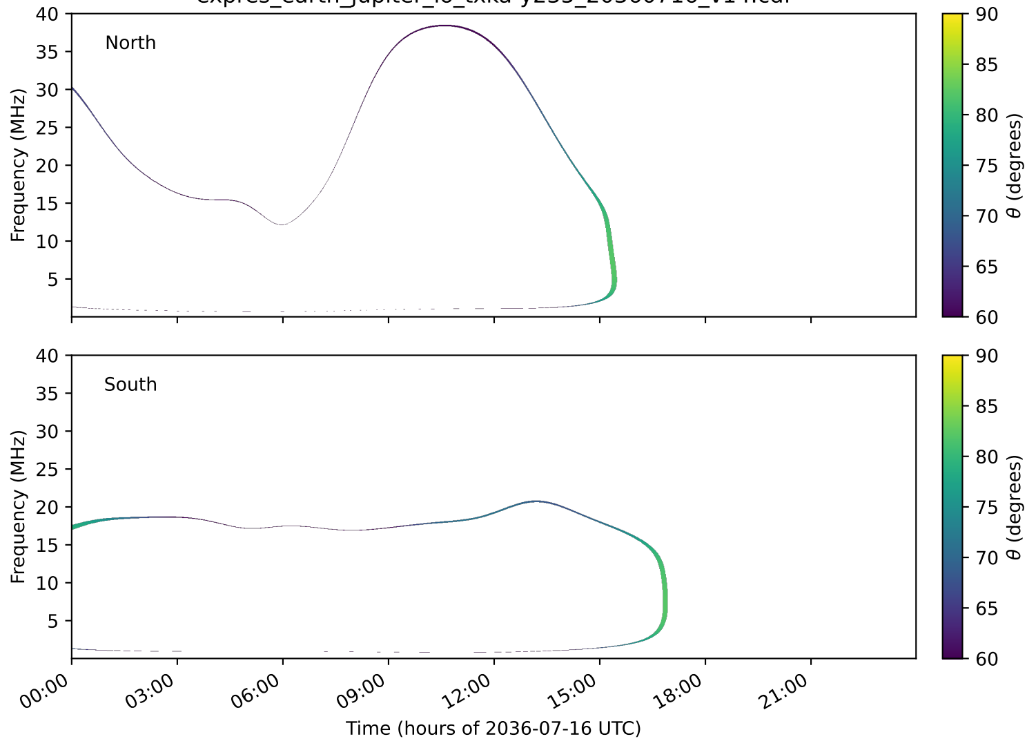
expres_earth_jupiter_io_txka-y235_20360716_v14.cdf
