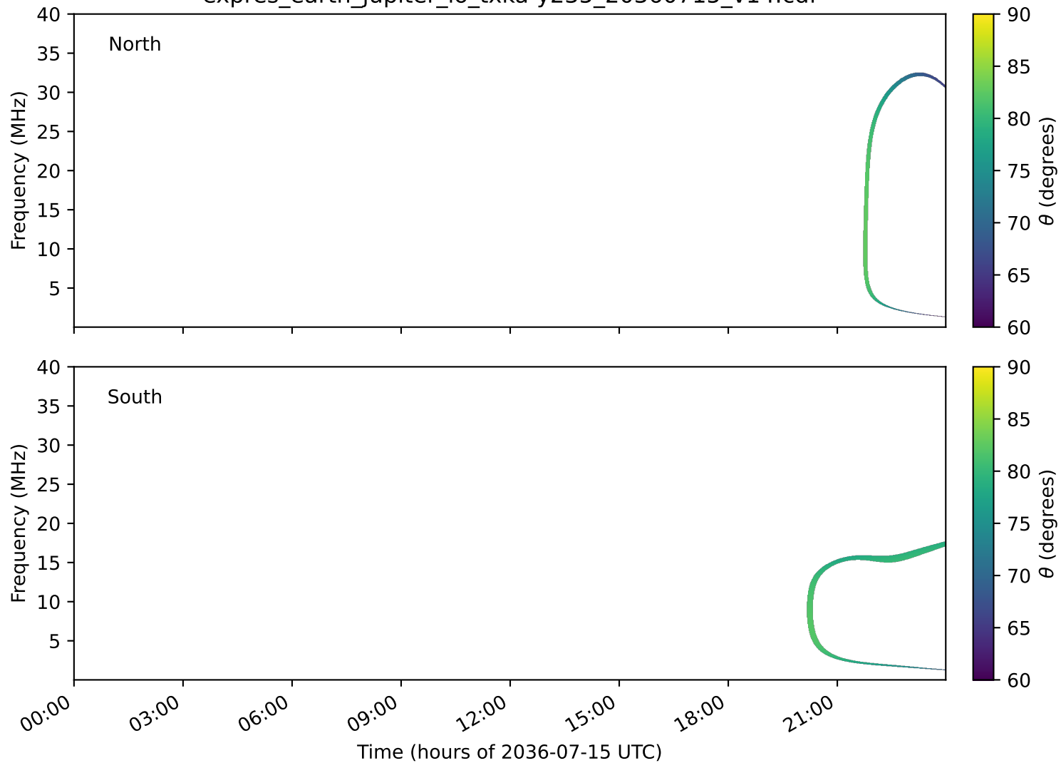
expres_earth_jupiter_io_txka-y235_20360715_v14.cdf
