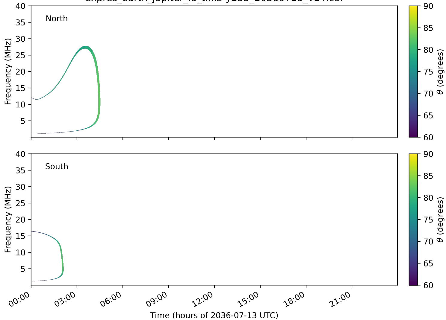
expres_earth_jupiter_io_txka-y235_20360713_v14.cdf
