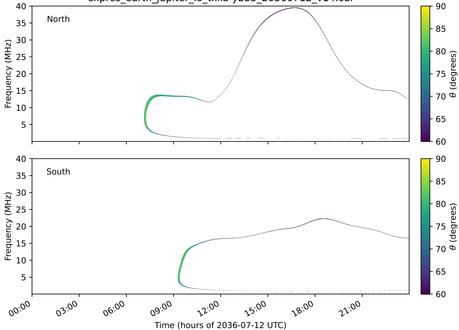
expres_earth_jupiter_io_txka-y235_20360712_v14.cdf
