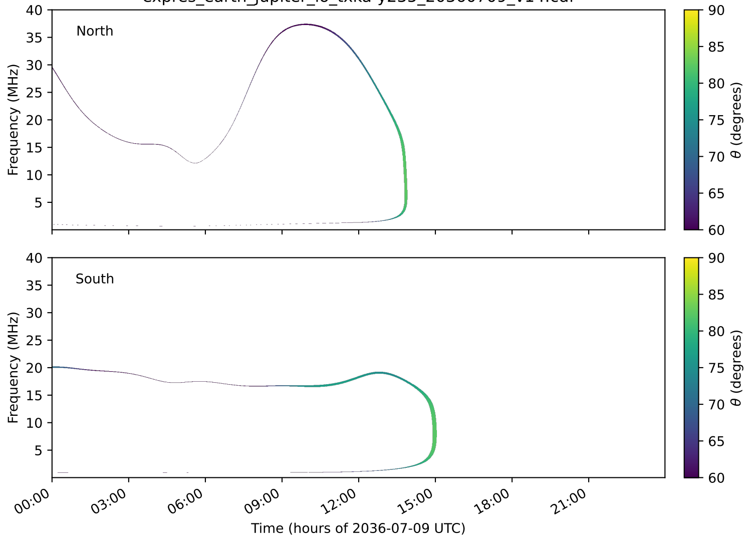
expres_earth_jupiter_io_txka-y235_20360709_v14.cdf
