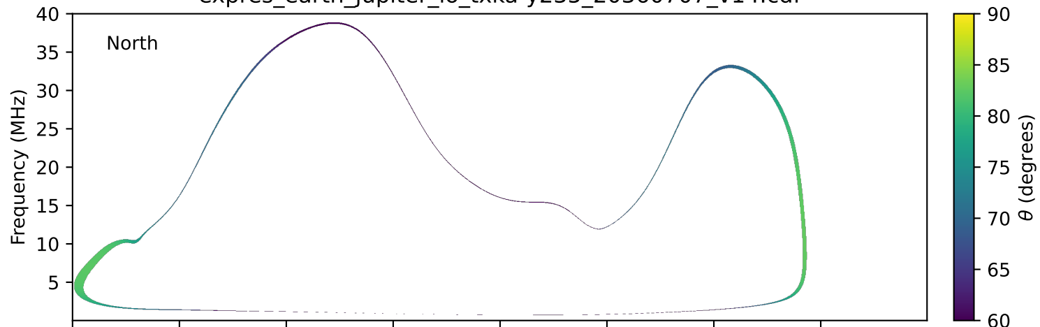
expres_earth_jupiter_io_txka-y235_20360707_v14.cdf
