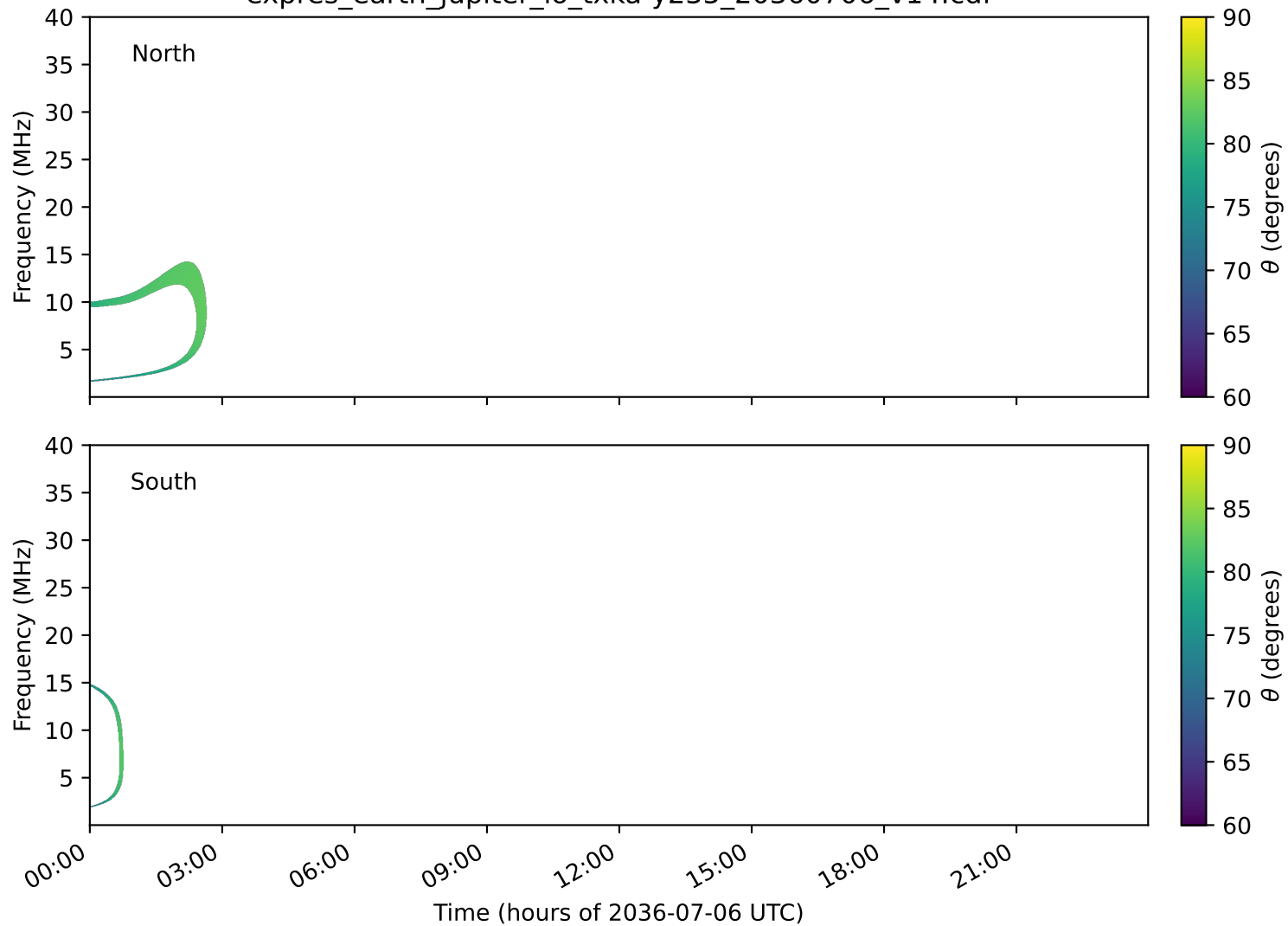
expres_earth_jupiter_io_txka-y235_20360706_v14.cdf
