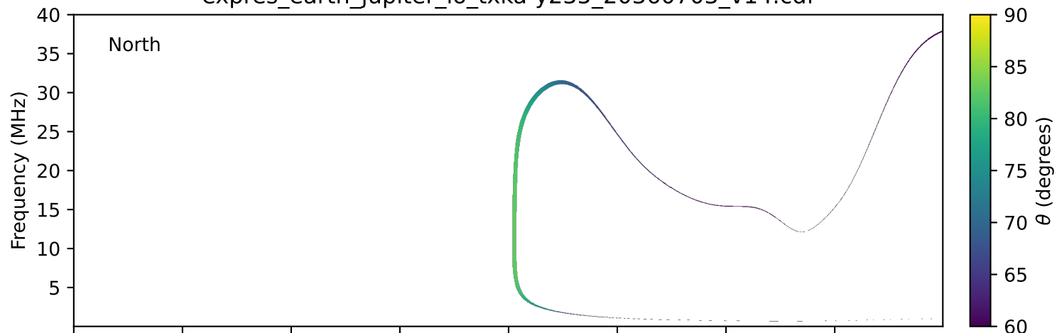
expres_earth_jupiter_io_txka-y235_20360703_v14.cdf
