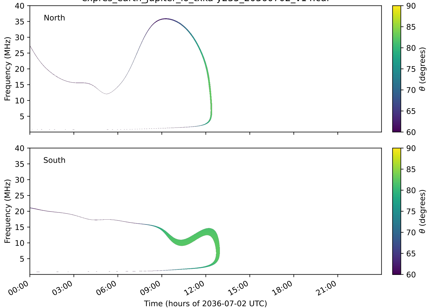
expres_earth_jupiter_io_txka-y235_20360702_v14.cdf
