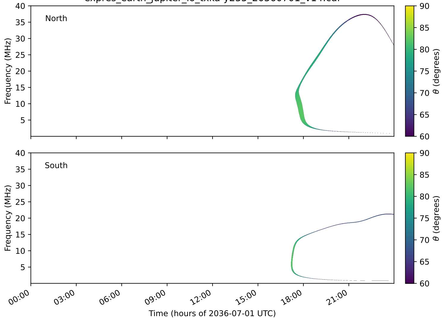
expres_earth_jupiter_io_txka-y235_20360701_v14.cdf
