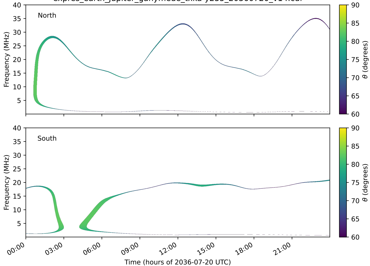
expres_earth_jupiter_ganymede_txka-y235_20360720_v14.cdf
