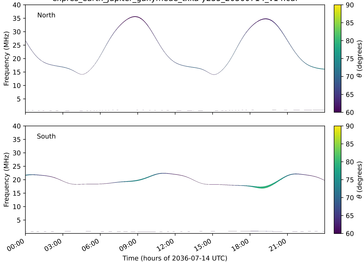
expres_earth_jupiter_ganymede_txka-y235_20360714_v14.cdf
