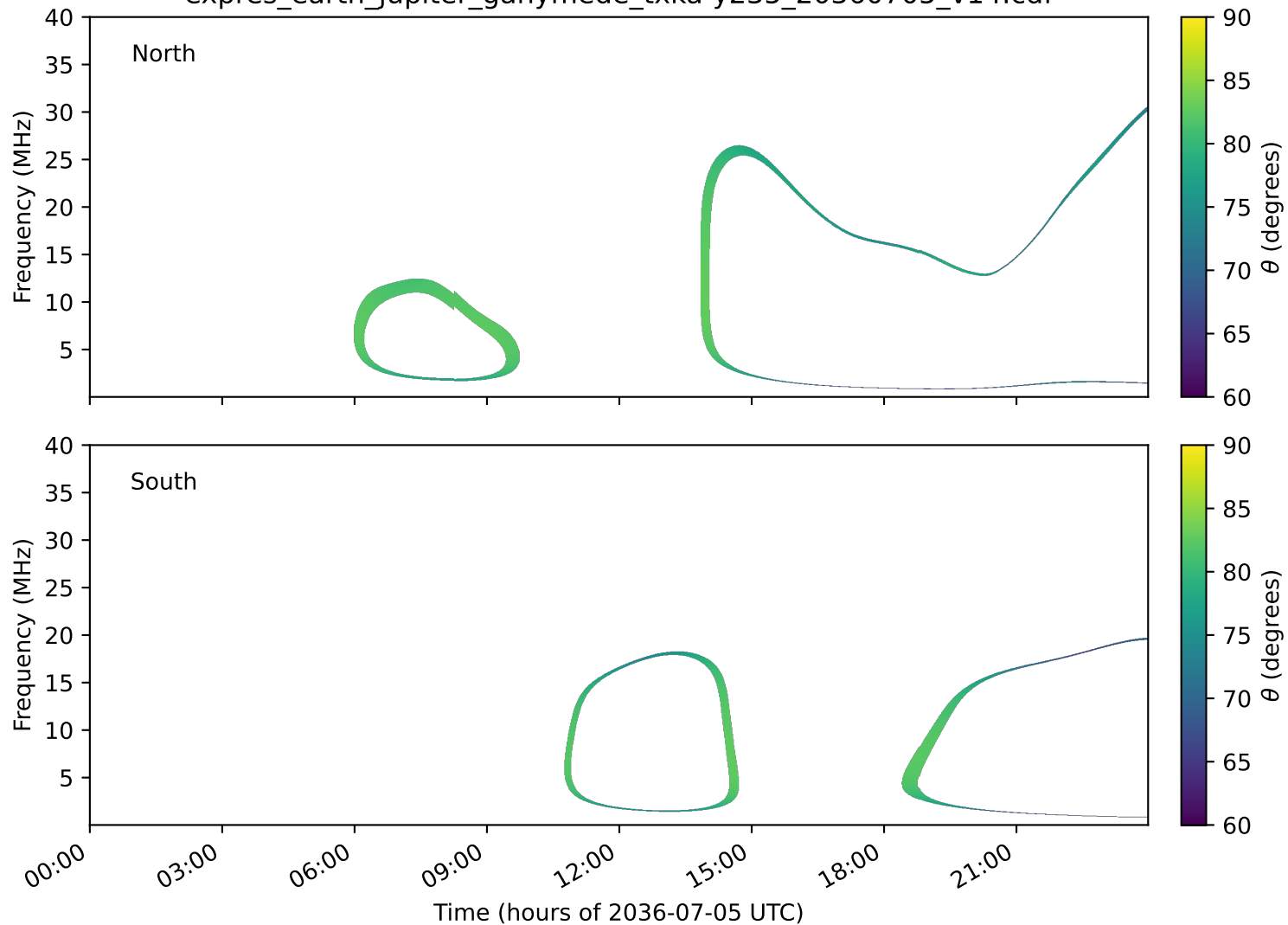
expres_earth_jupiter_ganymede_txka-y235_20360705_v14.cdf
