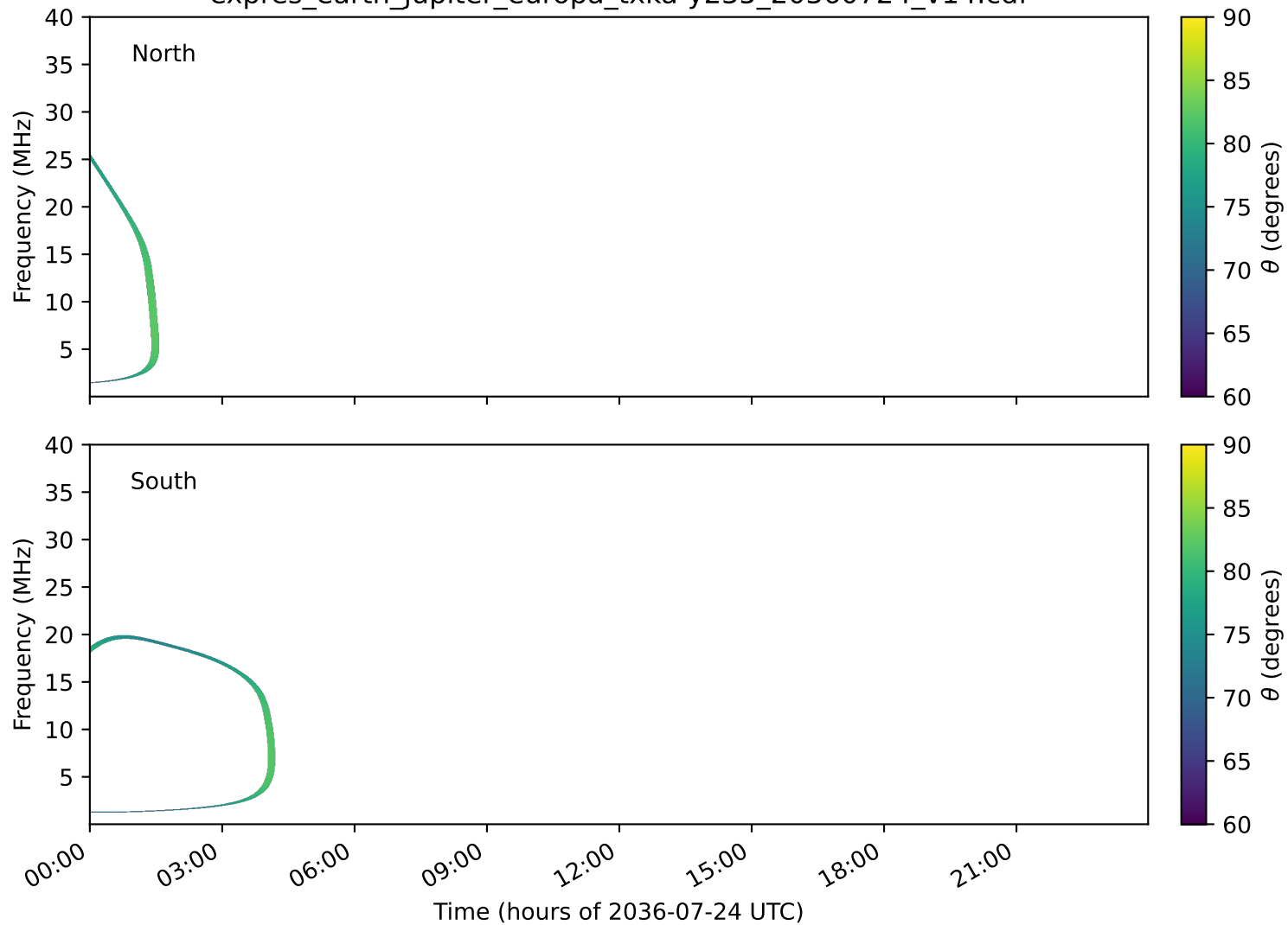
expres_earth_jupiter_europa_txka-y235_20360724_v14.cdf
