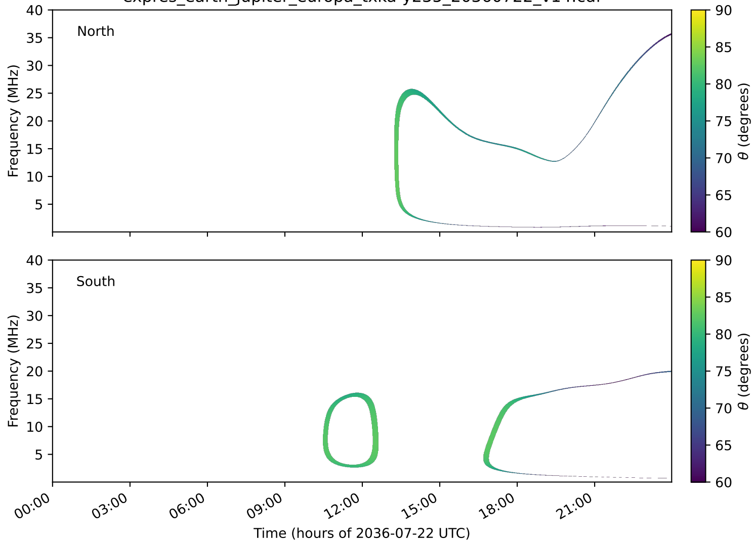
expres_earth_jupiter_europa_txka-y235_20360722_v14.cdf
