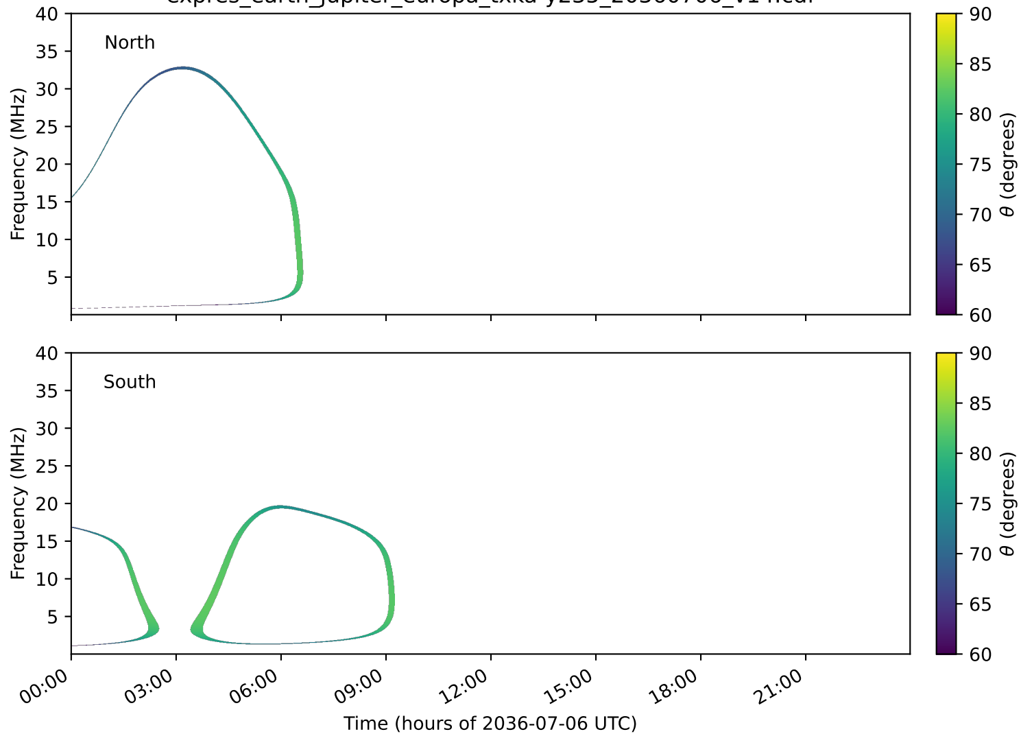
expres_earth_jupiter_europa_txka-y235_20360706_v14.cdf
